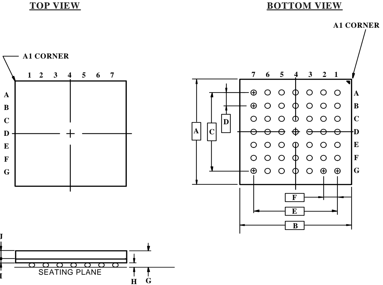
Figure 5: 49 Pin TFBGA Package
