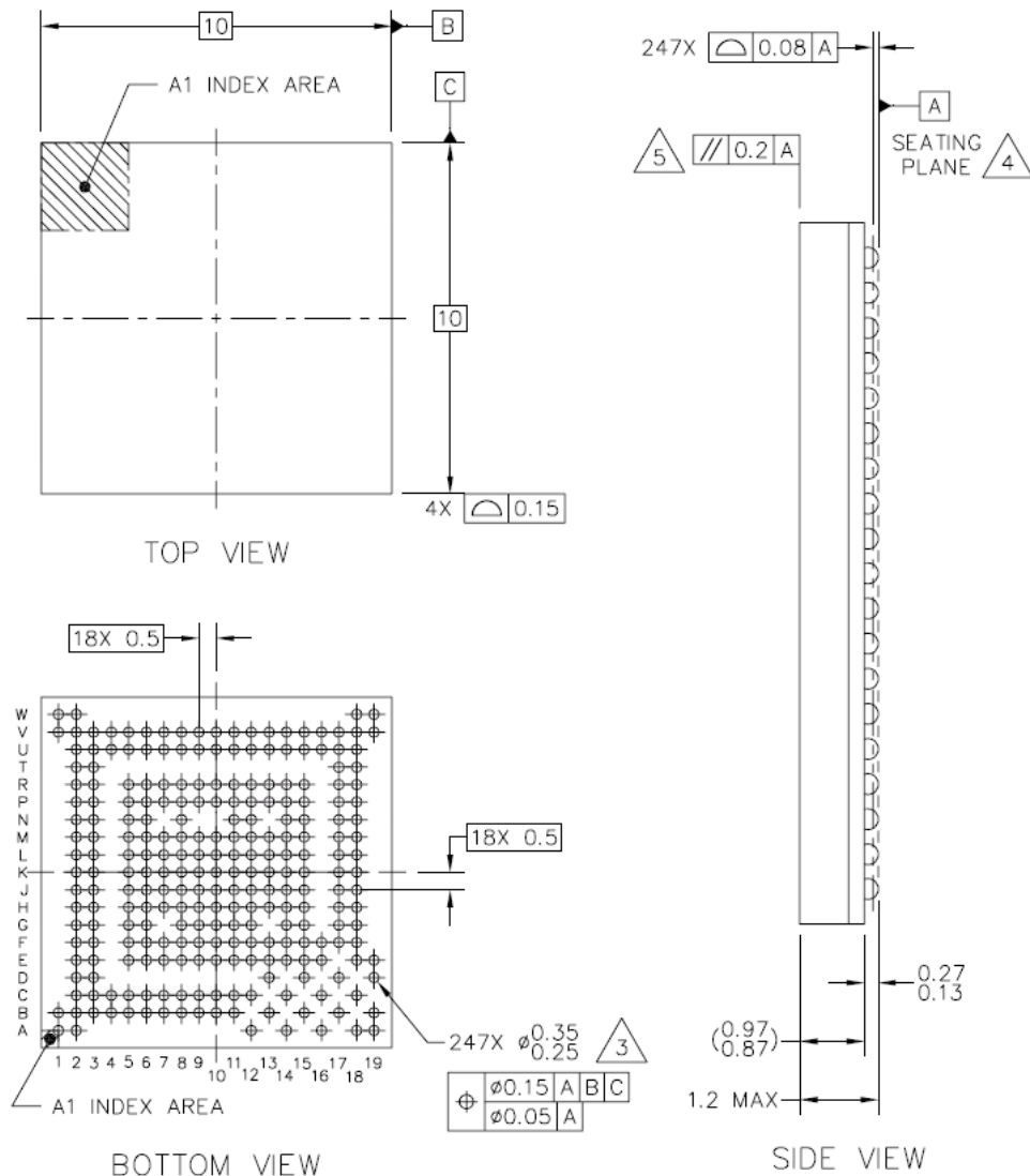
Figure 13. Package Drawing
